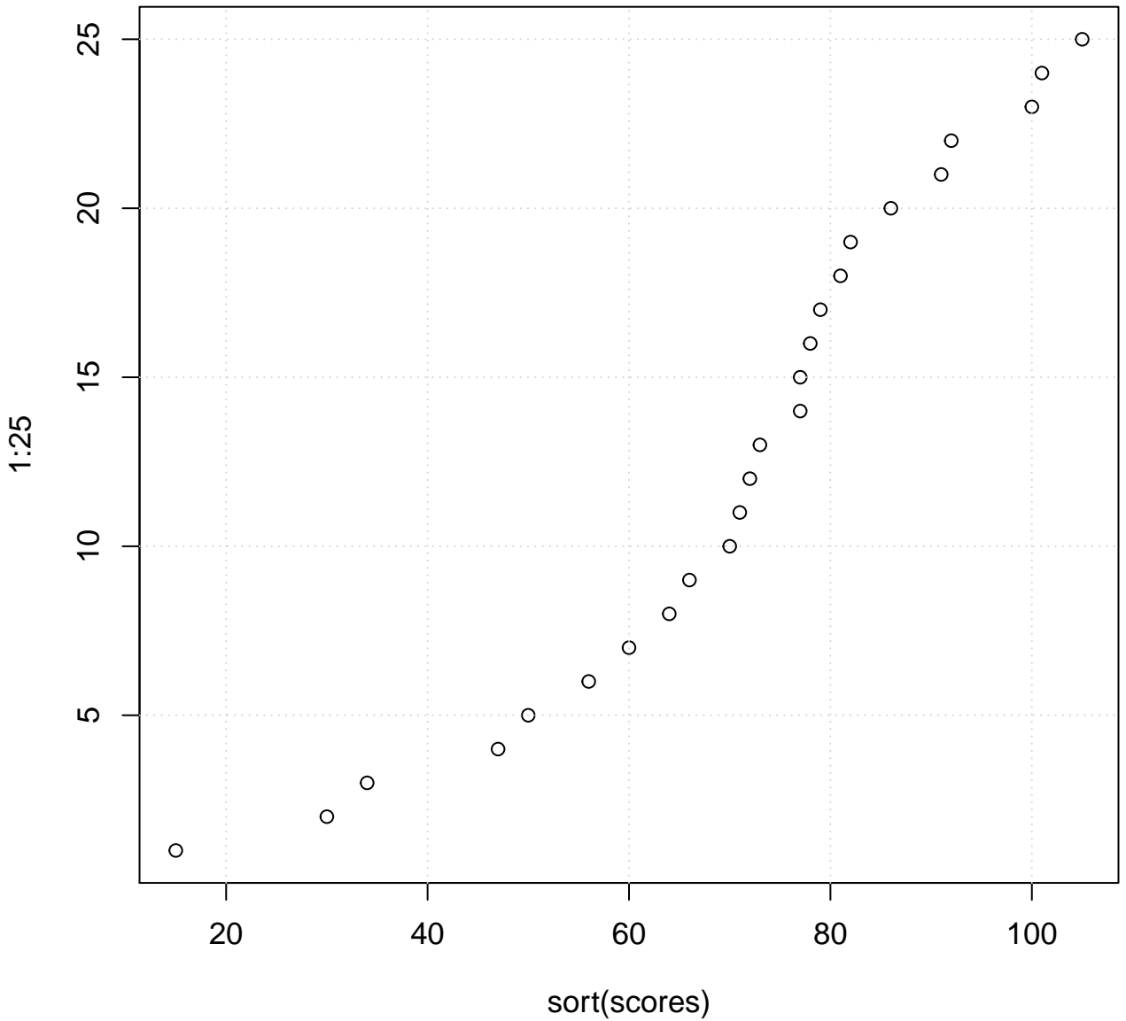
CDF of mid-term exam scores for 517
