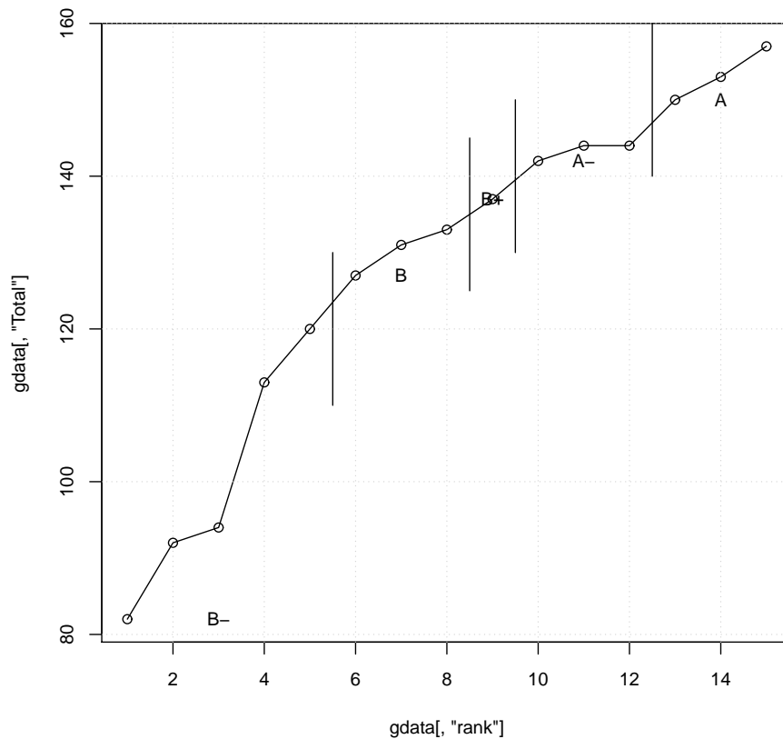
CDF of total point scores on ECO521 final exam
